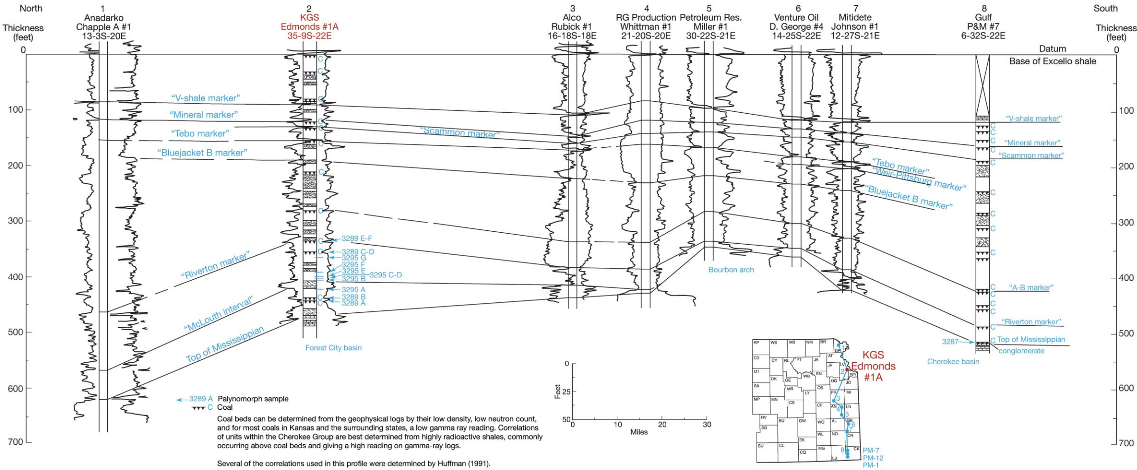
FIGURE 2—North-south profile of Cherokee Group in eastern Kansas. Portions of the profile are modified from Huffman (1991).
