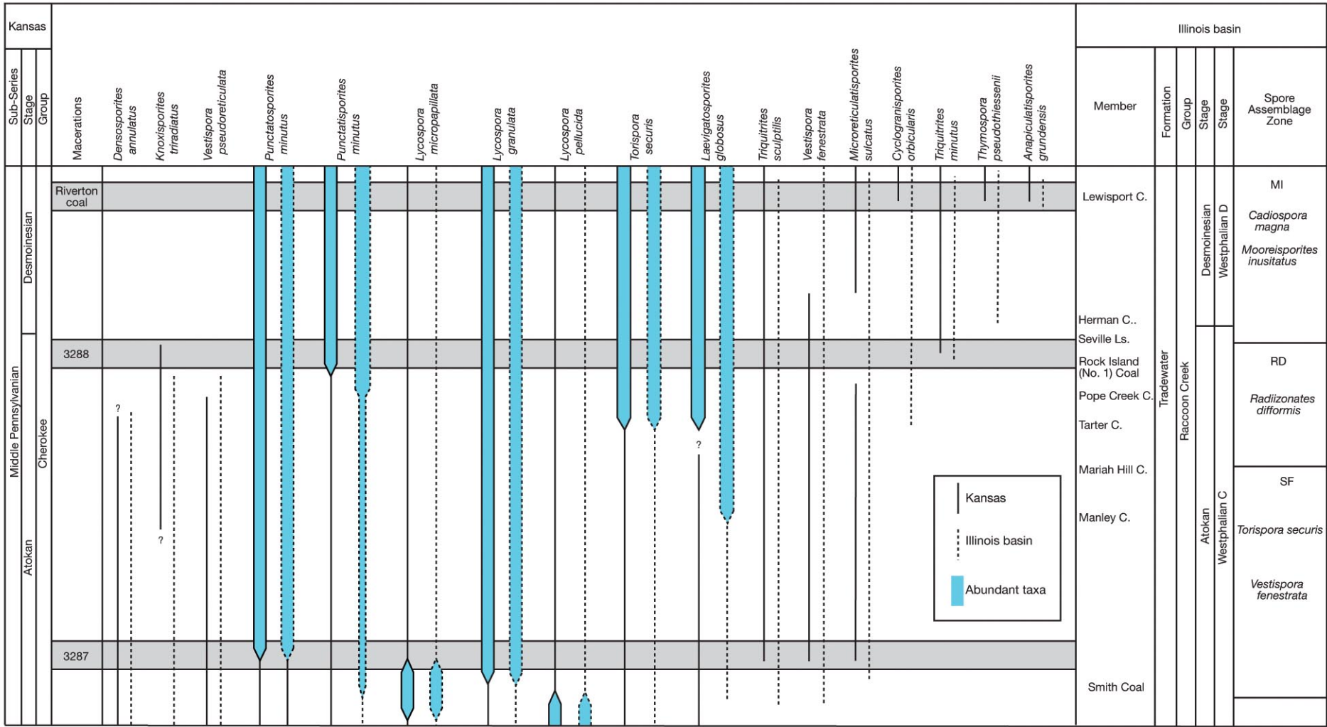
FIGURE 5—Chronostratigraphic ranges of selected spore species in oldest Pennsylvanian coal beds in the three cores drilled in Cherokee County, Kansas, compared with the range in the Illinois basin. Coals are shown in position relative to their ages.
