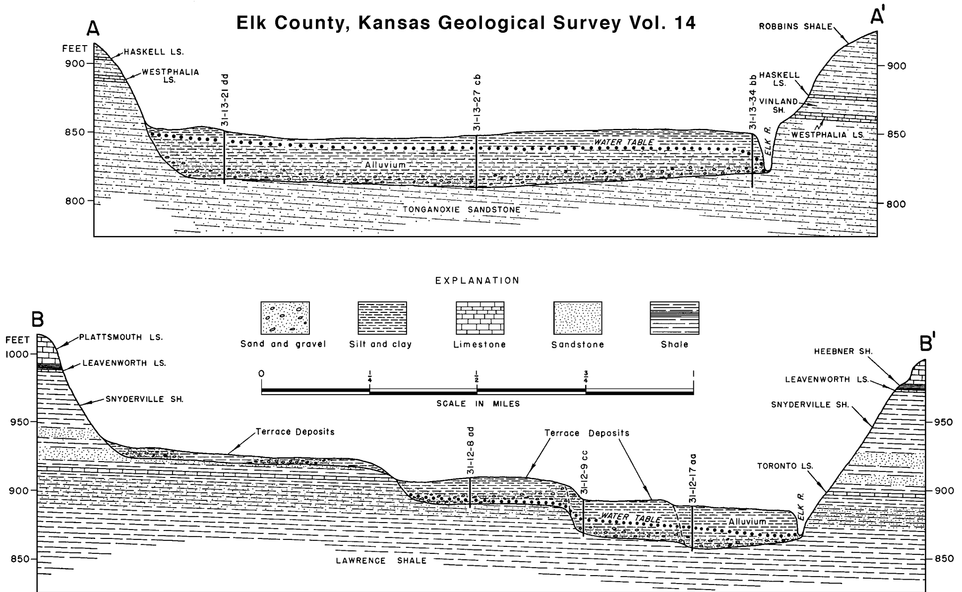
Figure 11—Geologic cross sections across Elk River Valley in Elk County, along lines A-A' and B-B'
