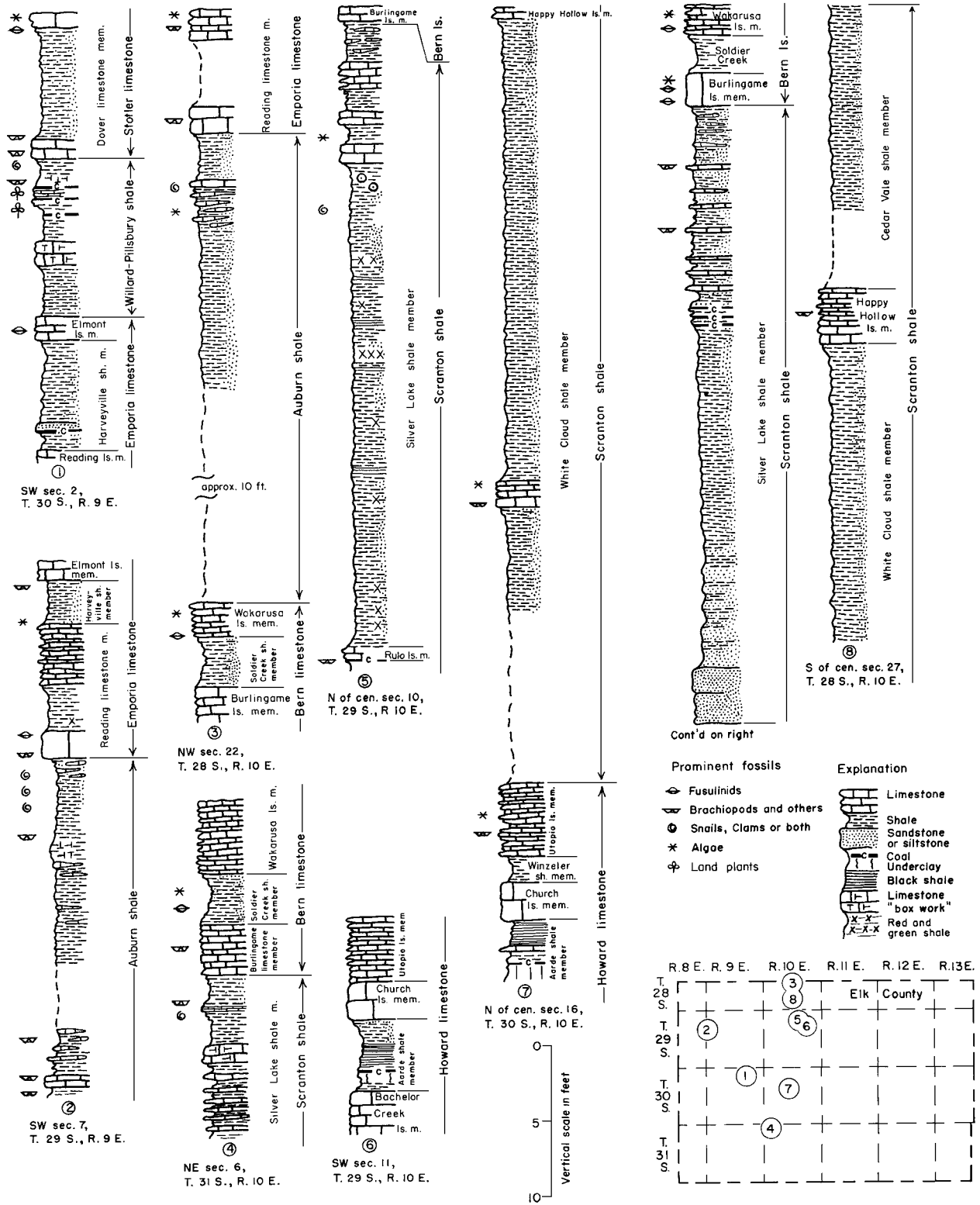
Figure 4 – Diagrammatic representation of outcropping upper Virgilian (Pennsylvanian) rocks.
