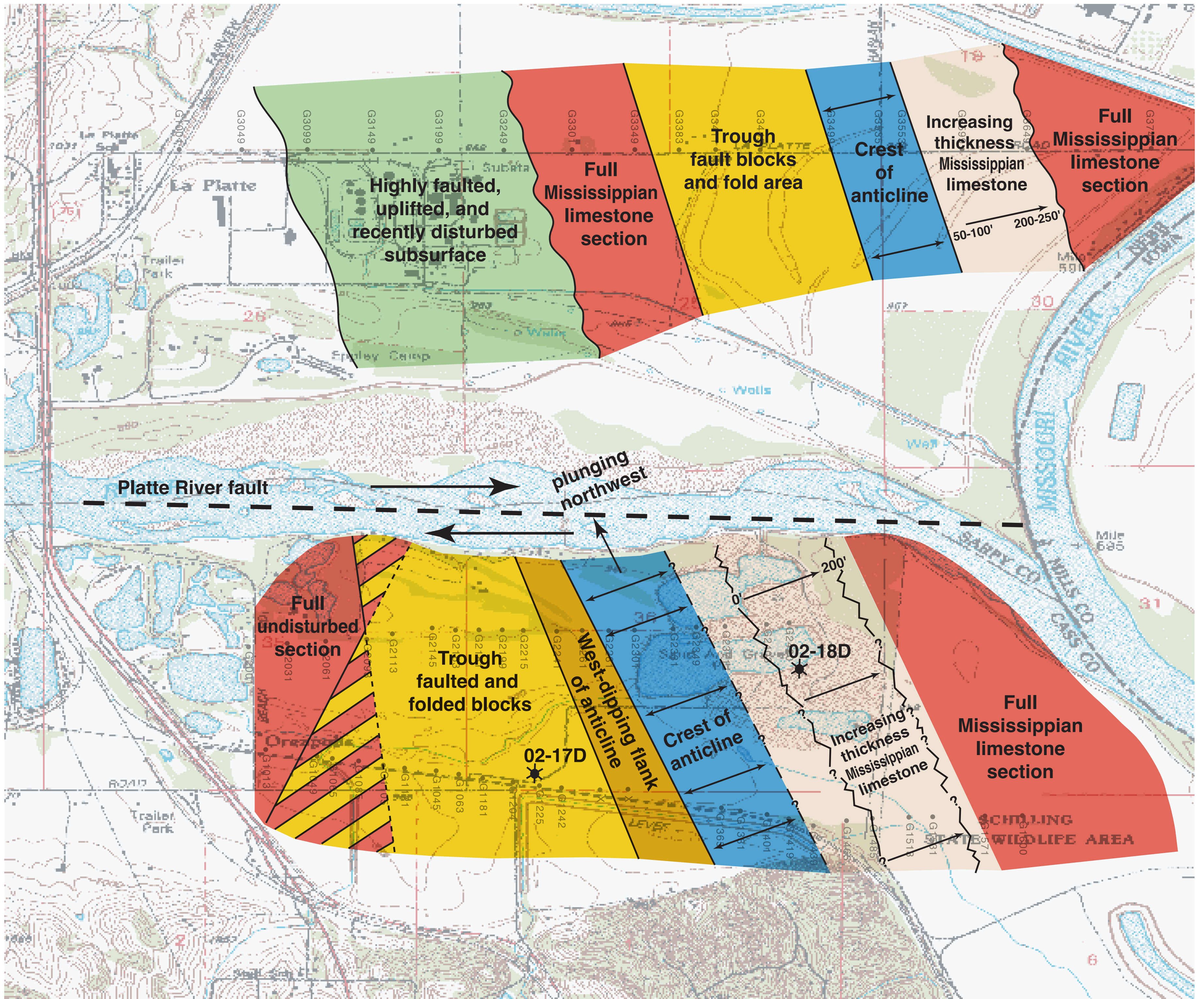
Figure 27. Site map with lines, stations, and major structures correlated between lines. Offset in anticline across Platte River is indicative of a right lateral strike-slip fault.
