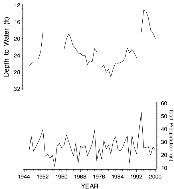
FIGURE 5--Depth to water in Osborne County, well 06S-12W-23-CDC-01 [31.8 ft (9.69 m) deep; unconsolidated Quaternary aquifer - alluvial terrace deposits], and precipitation at Cawker City (station 14137102).
