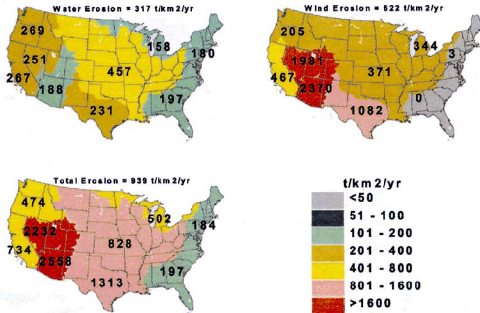
Plate 2. Estimated water, wind, and total erosion rates for each of the continental drainage provinces.
