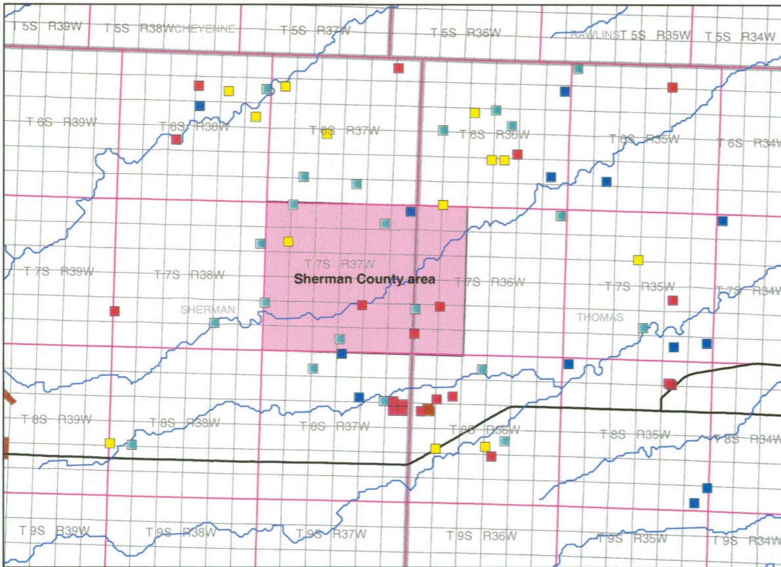
Figure 16 The sand and gravel fraction percentiles in the lower half of the combined Ogallala Formation – undifferentiated Quaternary, Sherman County study area. Drawn by Date File Name Projection Scale grh 02/10/03 Fig 16 Sand plus gravel frac L.mxd UTM Zone 14 NAD 1983 1:250,000
