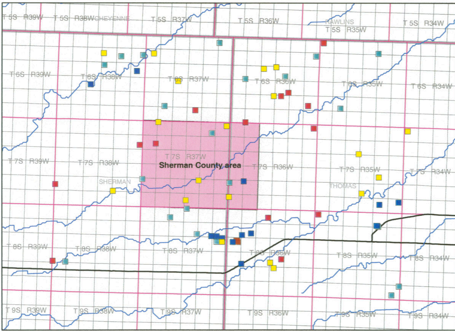
Figure 17 The coarse fraction percentiles in the lower half of the combined Ogallala Formation – undifferentiated Quaternary, Sherman County study area. Drawn by Date File Name Projection Scale grh 02/10/03 Fig 17 Coarse fraction L.mxd UTM Zone 14 NAD 1983 1:250,000
