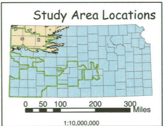
Figure 2 Distribution of the well-log data in the Sherman and Sheridan County study areas used in this investigation.
