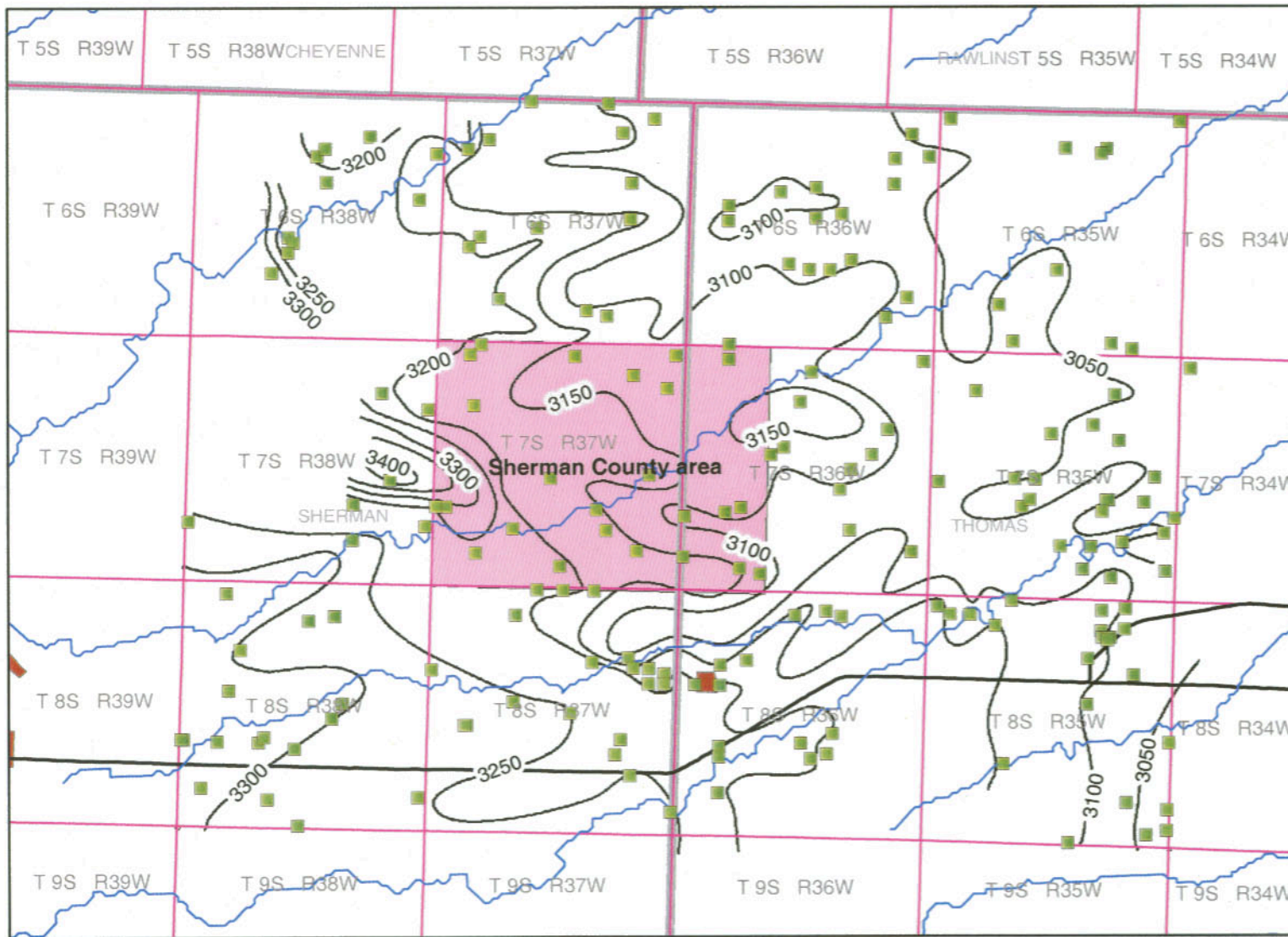
Figure 5 The bedrock surface elevation in the Sherman County study area. Drawn by Date File Name Projection Scale grh 02/10/03 Fig 05 Safe bedrock.mxd UTM Zone 14 NAD 1983 1:250,000
