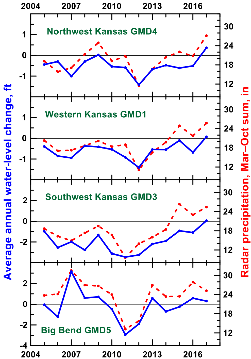
Figure 38—Mean annual water-level change and the radar precipitation (sum of March–October precipitation) for GMDs 4, 1, 3, and 5 during 2005–2017. The water-level change for a particular year is the water-level difference between the following year and that year for continuously measured wells for 2005–2017 and between the 2018 provisional winter value and the 2017 value. The blue lines represent the water-level change and the red dashed lines the radar precipitation. The ranges in the y-axes for water-level change in the upper two plots are half those of the lower two plots. The ranges in the y-axes for radar precipitation are the same for all four plots.
