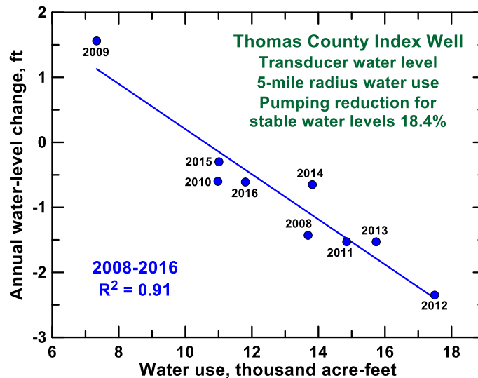
Figure 40—Correlation of annual water-level change based on transducer measurements in the Thomas County index well with annual water use within a 5 mi radius around the well during 2008–2016 ( p < 0.0001 ).
