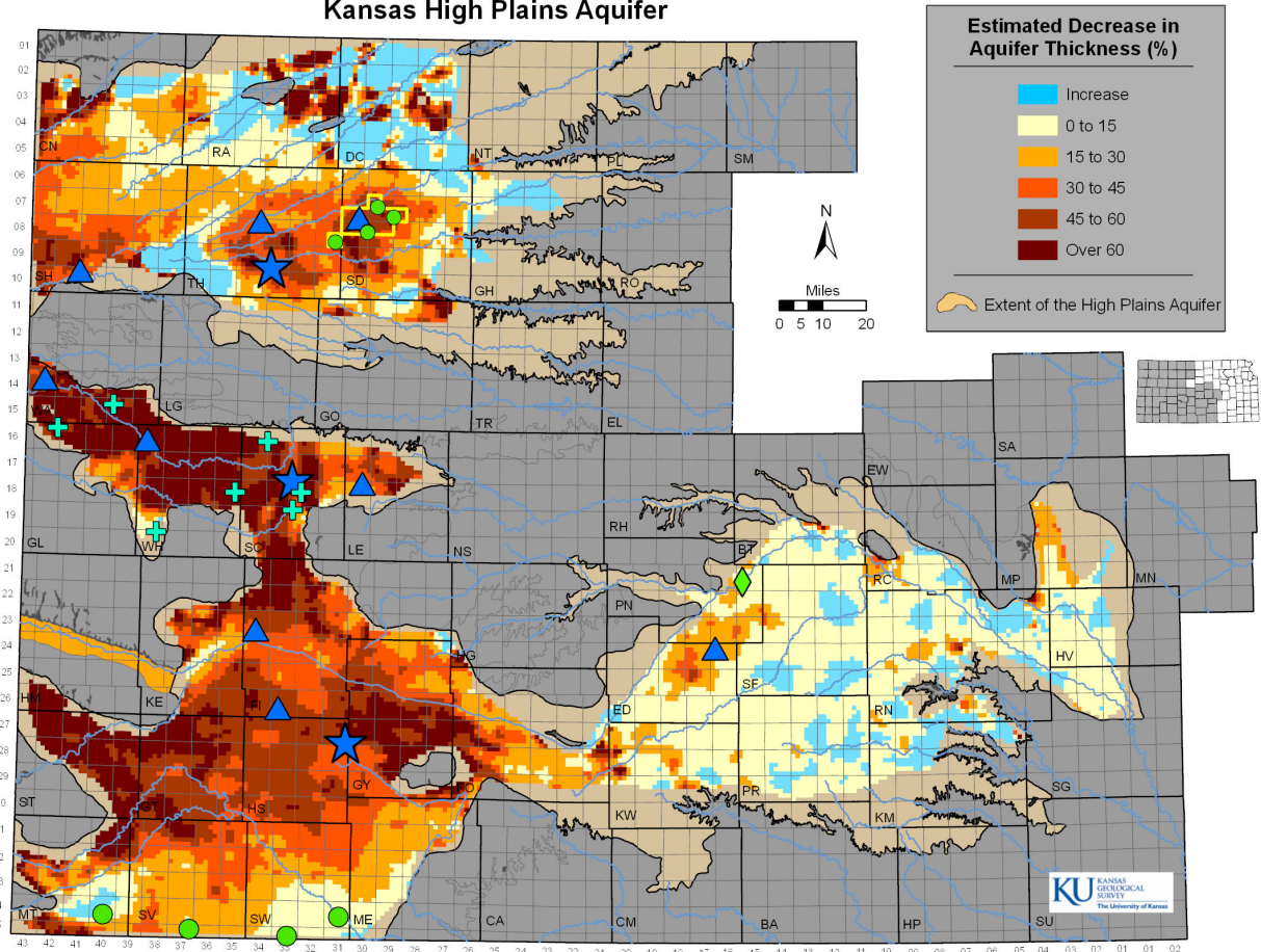
Figure 1—The Kansas portion of the High Plains aquifer, with aquifer and county boundaries shown. Each colored pixel represents one section (1 mi), coded for the degree of groundwater depletion from the beginning of large-scale development to the average of conditions in 2015–2017. The stars indicate the locations of the original three index well site, the triangles indicate additional telemetry-equipped wells, the circles are the index wells without telemetry equipment that are downloaded quarterly, the yellow polygon indicates the Sheridan-6 Local Enhanced Management Area, and the diamond indicates the location of the index well at Larned that will begin acquiring data in the summer of 2018. The plus signs are seven expansion wells that are monitored within GMD1.
