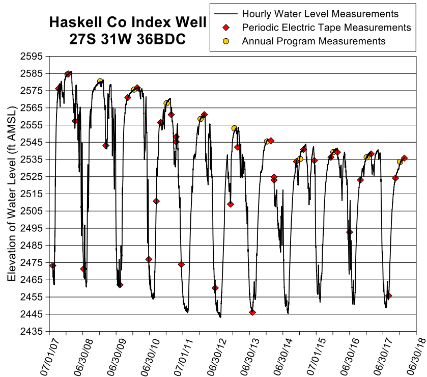
Figure 9—Haskell County index well hydrograph—total data run to 2/20/18. A water-level elevation of 2,445 ft corresponds to a depth to water of 392.85 ft below lsf. The top of the screen is 420 ft below lsf (elevation of 2,417.85 ft), and the bottom of the aquifer is 433 ft below lsf (elevation of 2,404.85 ft). The screen terminates 3 ft above the bottom of the aquifer. A sensor failure produced a break in monitoring from January to March 2014.
