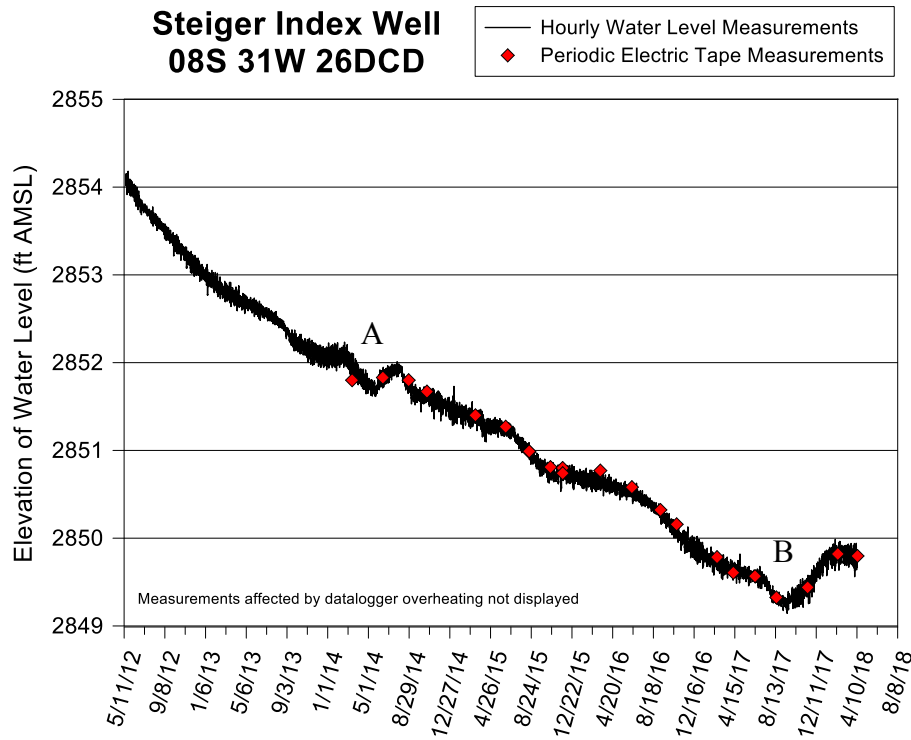
Figure 22—Steiger index well hydrograph—total data run to 4/11/18. A water-level elevation of 2,851 ft corresponds to a depth to water of 116.53 ft below Isf. The top of the 40 ft screen is 145 ft below Isf (elevation of 2,822.5 ft), and the bottom of the aquifer is 177 ft below Isf (elevation of 2,790.5 ft). A and B defined in text.
