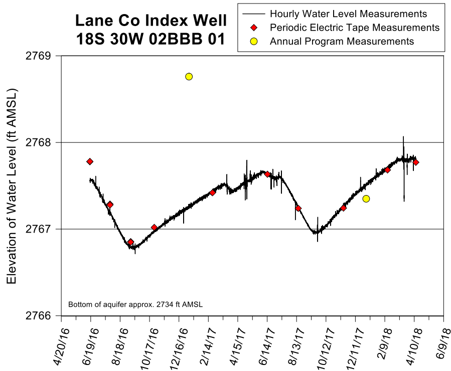
Figure 3—Lane County index well hydrograph—total data run to 4/13/18. A water-level elevation of 2,767 ft corresponds to a depth to water of 85 ft below land surface (lsf). The top of the screen is 105 ft below lsf (elevation of 2,747 ft), and the bottom of the aquifer is 118 ft below lsf (elevation of 2,734 ft). The screen terminates 3 ft above the bottom of the aquifer. The 2017 and, to a lesser extent, the 2018 annual water-level measurements appear to be in error.
