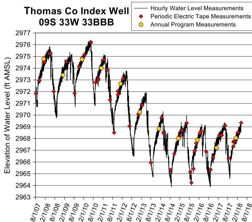
Figure 24—Thomas County index well hydrograph—total data run to 4/11/18. A water-level elevation of 2,968 ft corresponds to a depth to water of 219.56 ft below Isf. The top of the screen is 274 ft below Isf (elevation of 2,913.6 ft), and the bottom of the aquifer is 284 ft below Isf (elevation of 2,903.6 ft). The screen terminates at the bottom of the aquifer. No water-level data are available from 10/28/17 to 12/11/17 because of failure of sensor and backup sensor.
