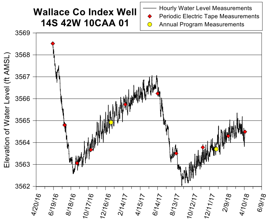
Figure 5—Wallace County index well hydrograph—total data run to 4/12/18. A water-level elevation of 3,565 ft corresponds to a depth to water of 263 ft below Isf. The top of the screen is 375 ft below Isf (elevation of 3,453 ft), and the bottom of the aquifer is 394 ft below Isf (elevation of 3,434 ft). The screen terminates 9 ft above the bottom of the aquifer.
