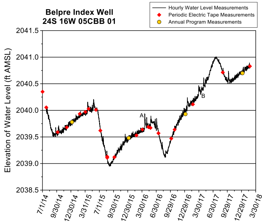
Figure 26—Belpre index well hydrograph—total data run to 2/21/18. A water-level elevation of 2,040 ft corresponds to a depth to water of 40 ft below Isf. The top of the 20 ft screen is 89 ft below Isf (elevation of 1,991 ft), and the bottom of the screen is 109 ft below Isf (elevation of 1,971 ft). The base of the aquifer is estimated to be 175–200 ft below Isf (elevation of 1,905–1,880 ft). A and B defined in text.
