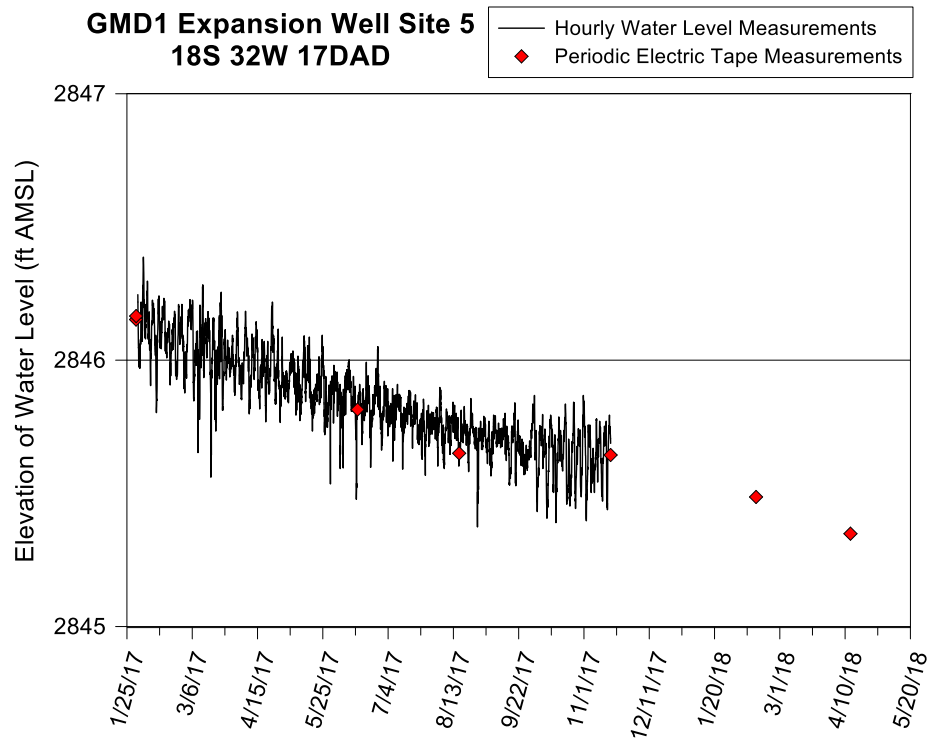
Figure 33—GMD1 Expansion Site 5 well hydrograph—total data run to 11/17/17 when battery died. A water-level elevation of 2,846 ft corresponds to a depth to water of 130 ft below lsf. Elevation of well bottom not known.
