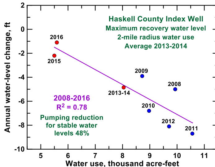
Figure 42—Correlation of change in maximum recovery water level based on transducer measurements in the Haskell County index well with annual water use within a 2 mi radius around the well during 2008–2016 ( p=0.0035 ). Red points designate values after the court-ordered shutdowns (see section 3.2.2); 2013 and 2014 values are averaged because of equipment failure at the time of the 2013 maximum recovery.
