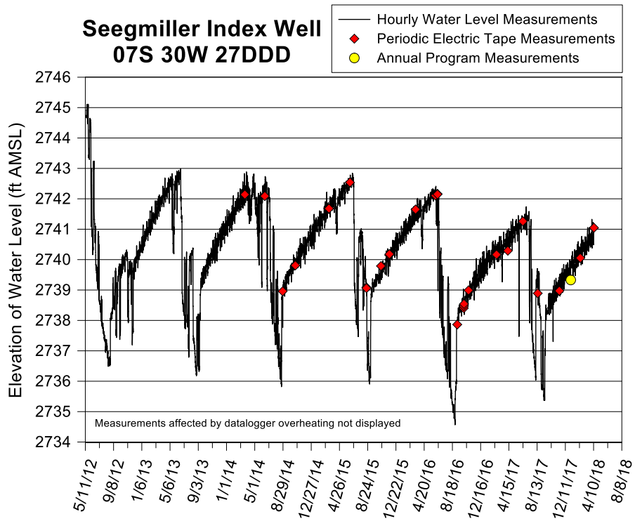
Figure 21—Seegmiller index well hydrograph—total data run to 4/11/18. A water-level elevation of 2,740 ft corresponds to a depth to water of 195.69 ft below Isf. The top of the 40 ft screen is 225 ft below Isf (elevation of 2,710.7 ft), and the bottom of the aquifer is 265 ft below Isf (elevation of 2,670.7 ft).
