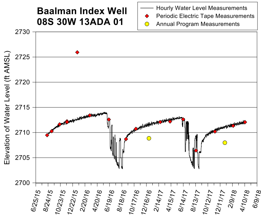
Figure 18—Baalman index well hydrograph—total data run to 4/11/18. A water-level elevation of 2,712 ft corresponds to a depth to water of 185 ft below Isf. The top of the 10 ft screen is 260 ft below Isf (elevation of 2,637 ft), and the bottom of the aquifer is 262 ft below Isf (elevation of 2,635 ft). The difference between the electric-tape and transducer measurements in January 2016 was caused by a malfunctioning electric tape.
