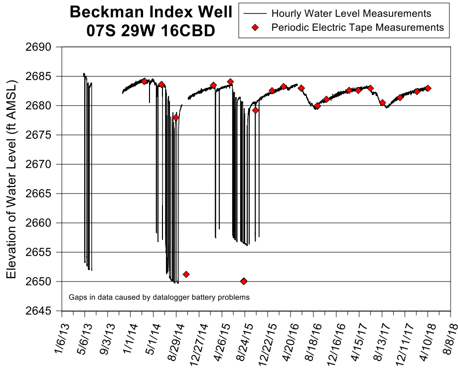
Figure 19—Beckman index well hydrograph—total data run to 4/11/18. A water-level elevation of 2,680 ft corresponds to a depth to water of 200.15 ft below lsf. The difference between the electric tape measurement in the summer of 2015 and the hourly measurements from the transducer is thought to be caused by a change in calibration specifications associated with the resumption of monitoring in late October 2014.
