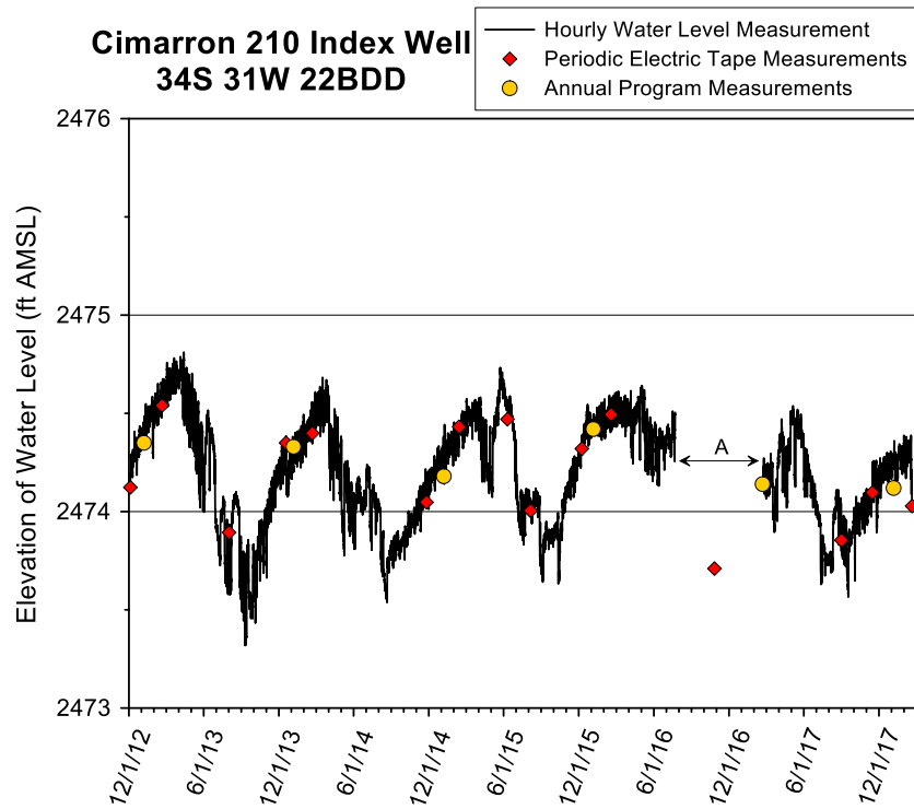
Figure 8—Cimarron 210 index well hydrograph—total data run to 2/19/18. A water-level elevation of 2,474 ft corresponds to a depth to water of 55.0 ft below Isf. The top of the 10 ft screen is 200 ft below Isf (elevation of 2,329 ft), and the bottom of the aquifer is 345 ft below Isf (elevation of 2,184 ft). A defined in text.
