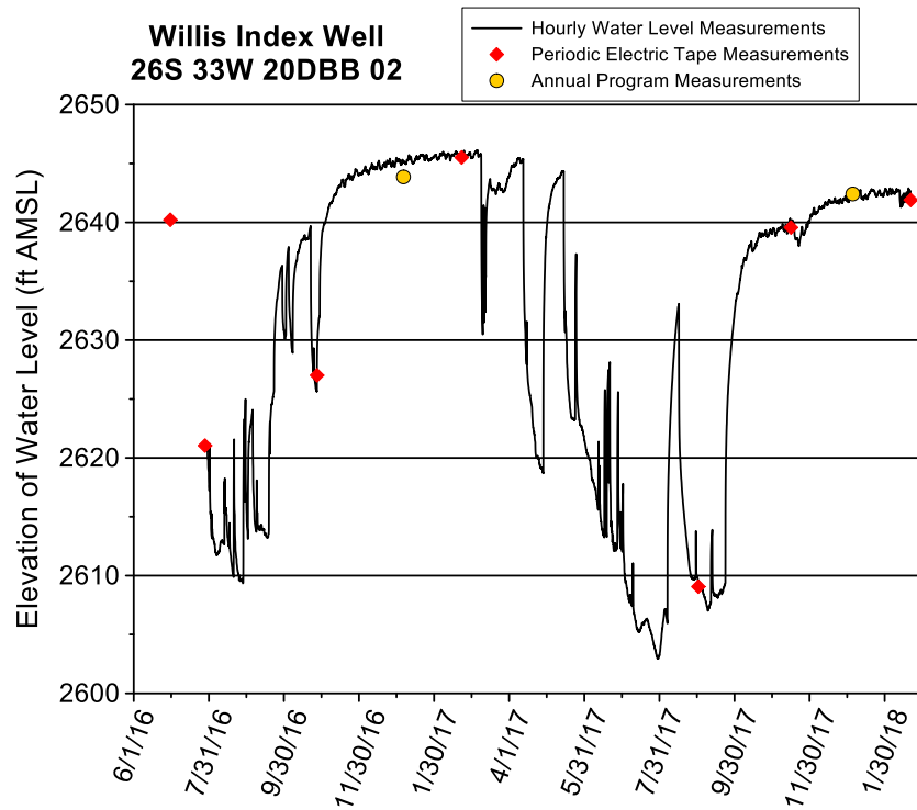
Figure 15—Willis Water Technology Farm index well hydrograph—total data run to 2/20/18. A water-level elevation of 2,640 ft corresponds to a depth to water of 300 ft below Isf. The top of the 220 ft screen is 262 ft below Isf (elevation of 2,678 ft), and the bottom of the aquifer is 502 ft below Isf (elevation of 2,438 ft). The first electric tape measurement was taken before continuous monitoring began.
