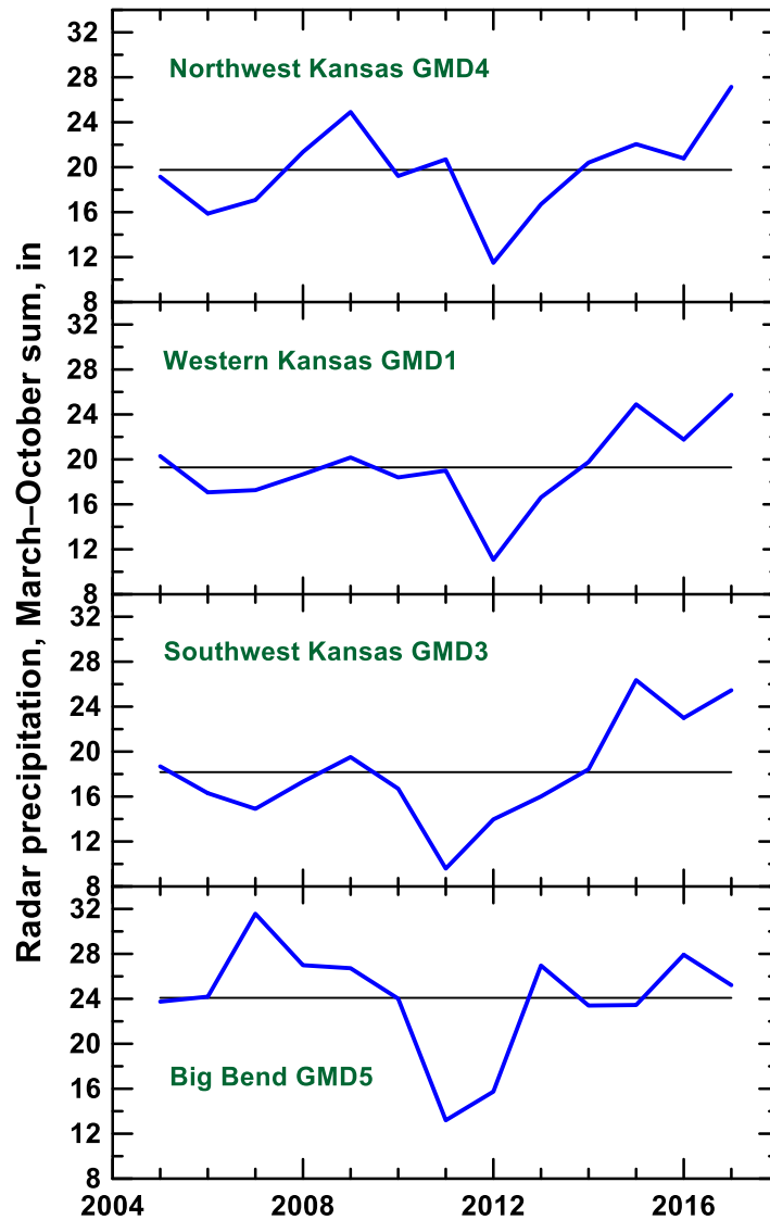
Figure 35—Radar precipitation versus time (blue line) for 2005–2017 for GMDs 4, 1, 3, and 5. Solid black line is the average precipitation for the period.
