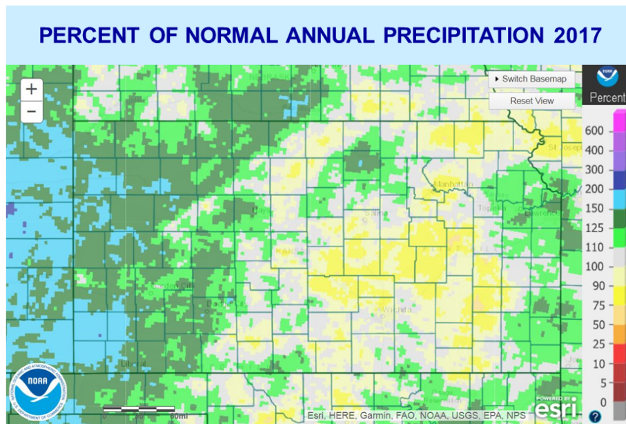
Figure 34—Percent of normal radar precipitation for Kansas in 2017. County lines and the state boundary (bolded) are displayed.
