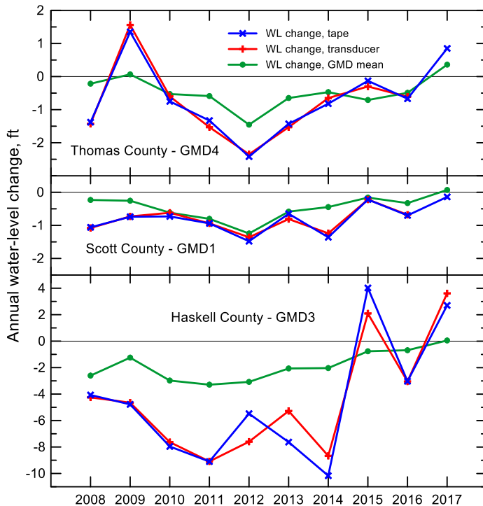
Figure 39—Annual winter water-level changes in the original three index wells and the mean annual changes in the three GMDs in western Kansas in which they are located. Note the different y-axis range for Haskell County versus that for Thomas and Scott counties; suspect 2013 tape measurement at the Haskell index well causes the 2012 and 2013 tape water-level change values to be markedly different from those based on the transducer measurements.
