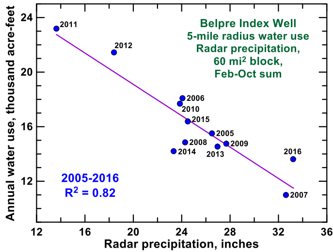
Figure 37—Correlation of annual total groundwater use with radar precipitation at the Colby, SC-8, and Belpre wells for 2008–2016.
