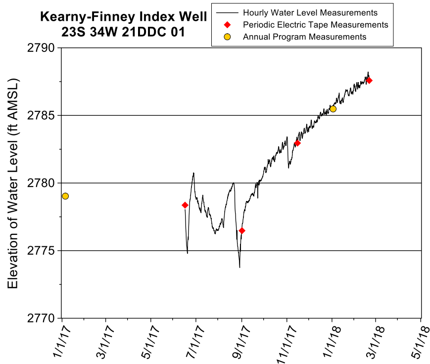
Figure 12—Kearny-Finney index well hydrograph—total data run to 2/20/18. A water-level elevation of 2,788 ft corresponds to a depth to water of 173 ft below lsf. Nominal bottom of well is 300 ft below lsf (elevation of 2,661 ft), but the well is currently filled with sediments to 266 ft below lsf (elevation of 2,695 ft).
