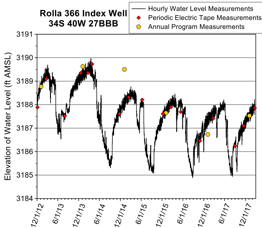
Figure 14—Rolla 366 index well hydrograph—total data run to 2/19/18. A water-level elevation of 3,188 ft corresponds to a depth to water of 187 ft below Isf. The top of the 10 ft screen is 356 ft below Isf (elevation of 3,019 ft), and the bottom of the aquifer is 399 ft below Isf (elevation of 2,976 ft). Note the suspect 2015 and 2017 annual program measurements.
