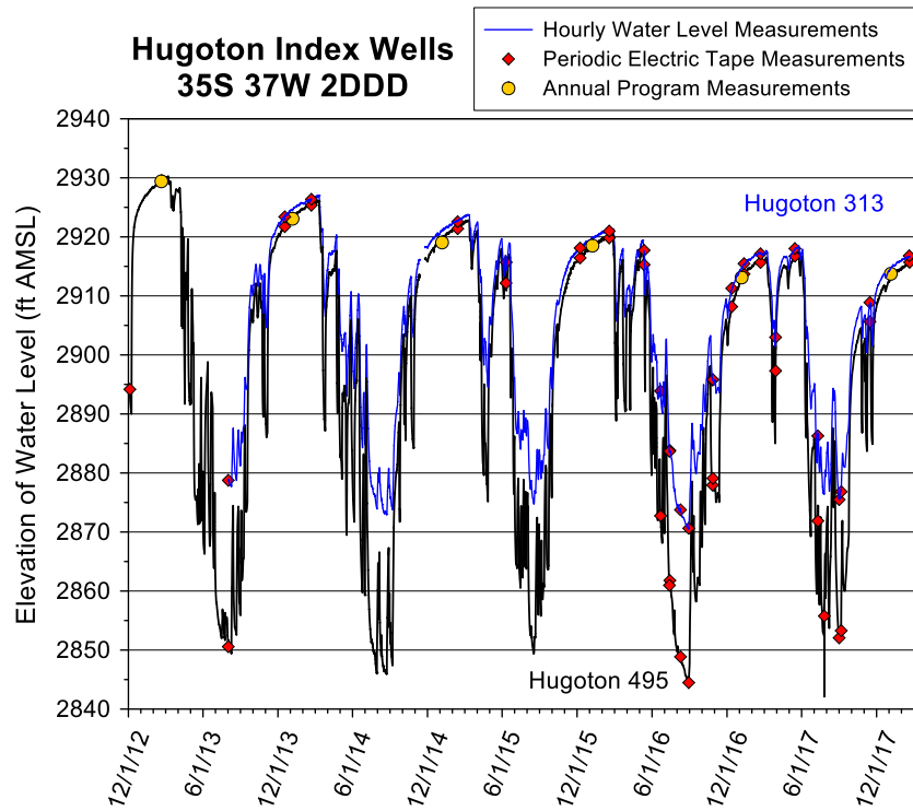
Figure 10—Hydrographs of Hugoton index wells—total data run to 2/19/18. A water-level elevation of 2,930.0 ft corresponds to a depth to water of 170.0 ft below Isf. For the Hugoton 495 well, the top of the 10 ft screen is 485 ft below Isf (elevation of 2,615 ft). For the Hugoton 313 well, the top of the 10 ft screen is 303 ft below Isf (elevation of 2,797 ft). Bottom of the aquifer is 635 ft below Isf (elevation of 2,465 ft).
