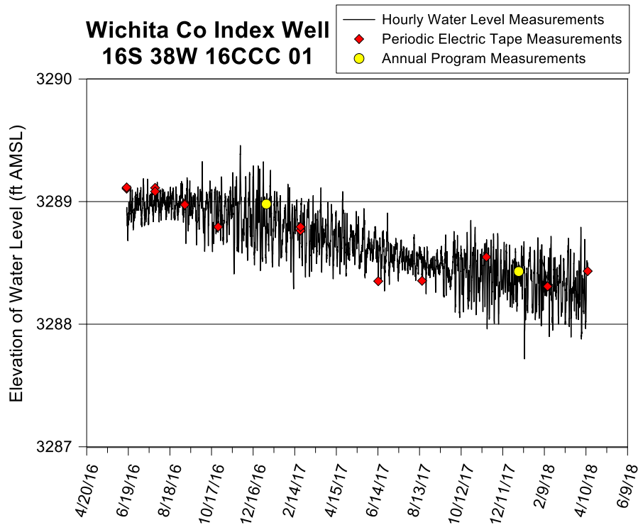
Figure 6—Wichita County index well hydrograph—total data run to 4/12/18. A water-level elevation of 3,289 ft corresponds to a depth to water of 159 ft below lsf. The top of the screen is 175 ft below lsf (elevation of 3,273 ft), and the bottom of the aquifer is 190 ft below lsf (elevation of 3,258 ft). The screen terminates 5 ft above the bottom of the aquifer.
