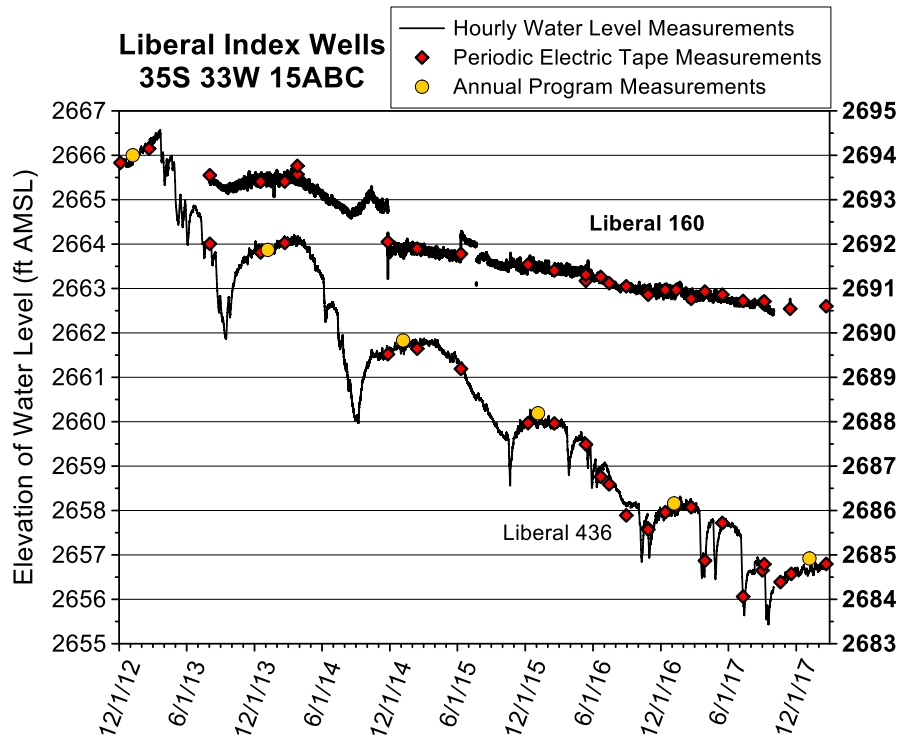
Figure 13—Hydrographs of Liberal index wells—total data run to 2/19/18. The Liberal 436 plot corresponds to the left y-axis. A water-level elevation of 2,664 ft corresponds to a depth to water of 157 ft below Isf. The top of the 10 ft screen is 426 ft below Isf (elevation of 2,395 ft). The Liberal 160 plot corresponds to the right y-axis. A water-level elevation of 2,692 ft corresponds to a depth to water of 129 ft below Isf. The top of the 20 ft screen is 140 ft below Isf (elevation of 2,681 ft). Bottom of the aquifer is 576 ft below Isf (elevation of 2,245 ft). A sensor failed at Liberal 160 well on November 16, 2017. Pre-2017 gaps in hydrograph for Liberal 160 were discussed in a previous report (Butler et al., 2017).
