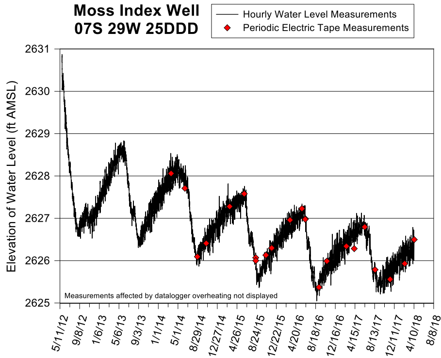
Figure 20—Moss index well hydrograph—total data run to 4/11/18. A water-level elevation of 2,627 ft corresponds to a depth to water of 191.44 ft below Isf. The top of the 40 ft screen is 205 ft below Isf (elevation of 2,613.4 ft), and the bottom of the aquifer is 243 ft below Isf (elevation of 2,575.4 ft).
