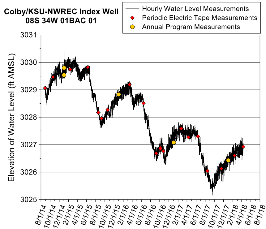
Figure 17—Colby index well hydrograph—total data run to 4/11/18. A water-level elevation of 3,029 ft corresponds to a depth to water of 148 ft below Isf. Total depth of the well is 175 ft below Isf (elevation of 3,002 ft). The screened interval extends from 156–175 ft below Isf. The base of the aquifer is estimated to be 250–300 ft below Isf (Butler et al., 2017).
