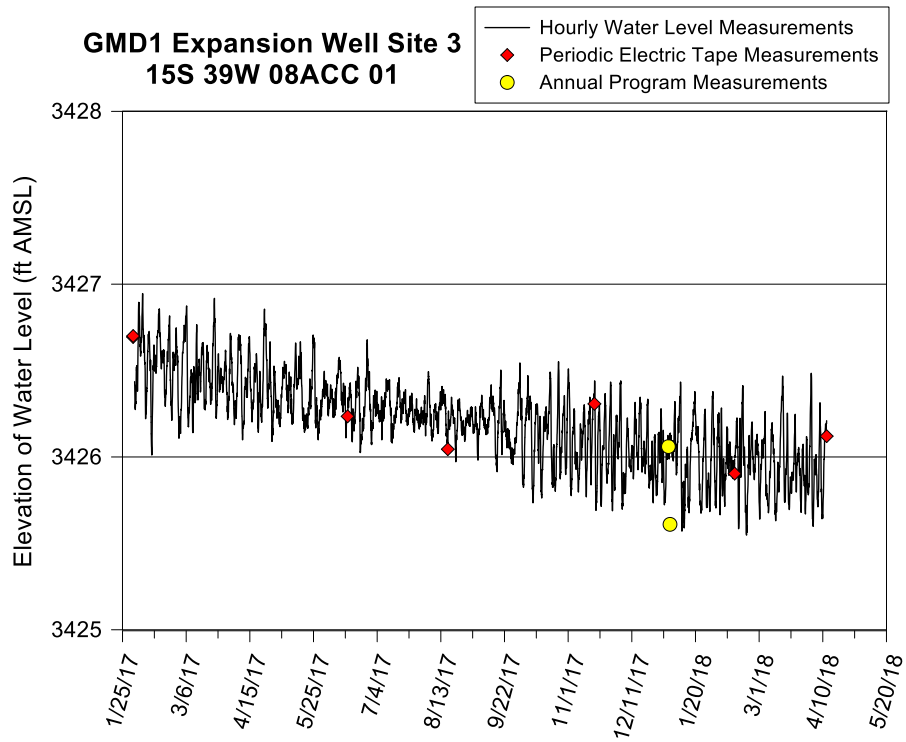
Figure 31—GMD1 Expansion Site 3 well hydrograph—total data run to 4/12/18. A water-level elevation of 3,426 ft corresponds to a depth to water of 197 ft below lsf. Bottom of well is 219.9 ft below lsf (elevation of 3,403.1 ft).
