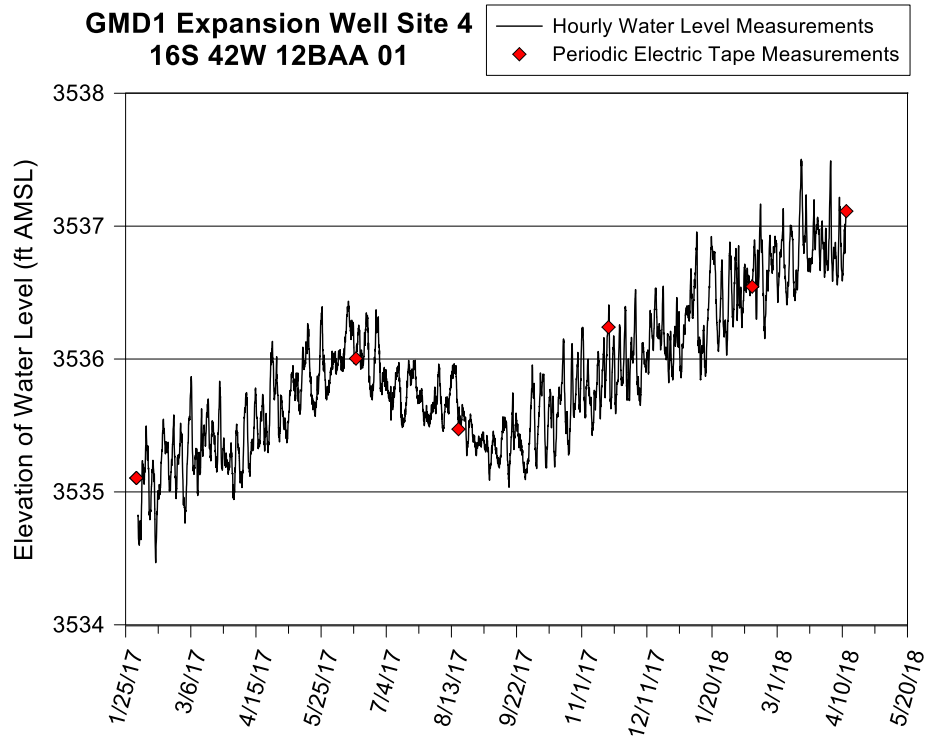
Figure 32—GMD1 Expansion Site 4 well hydrograph—total data run to 4/12/18. A water-level elevation of 3,537 ft corresponds to a depth to water of 236 ft below lsf. Bottom of well is 264.5 ft below lsf (elevation of 3,508.5 ft).
