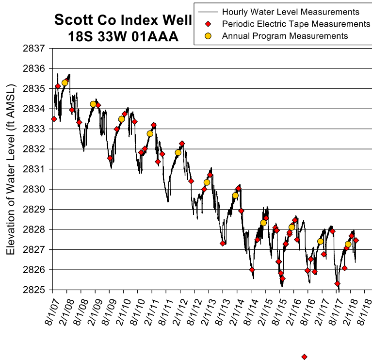
Figure 4—Scott County index well hydrograph—total data run to 4/12/18. A water-level elevation of 2,829 ft corresponds to a depth to water of 138.15 ft below Isf. The top of the screen is 215 ft below Isf (elevation of 2,752.15 ft), and the bottom of the aquifer is 223 ft below Isf (elevation of 2,744.15 ft). The screen terminates 2 ft below the bottom of the aquifer. Transducer data has been adjusted for change in position as described in a previous annual report (Butler, Whittemore, Reboulet et al., 2016). Electric-tape measurement plotted below the graph appears to have been a transcription error.
