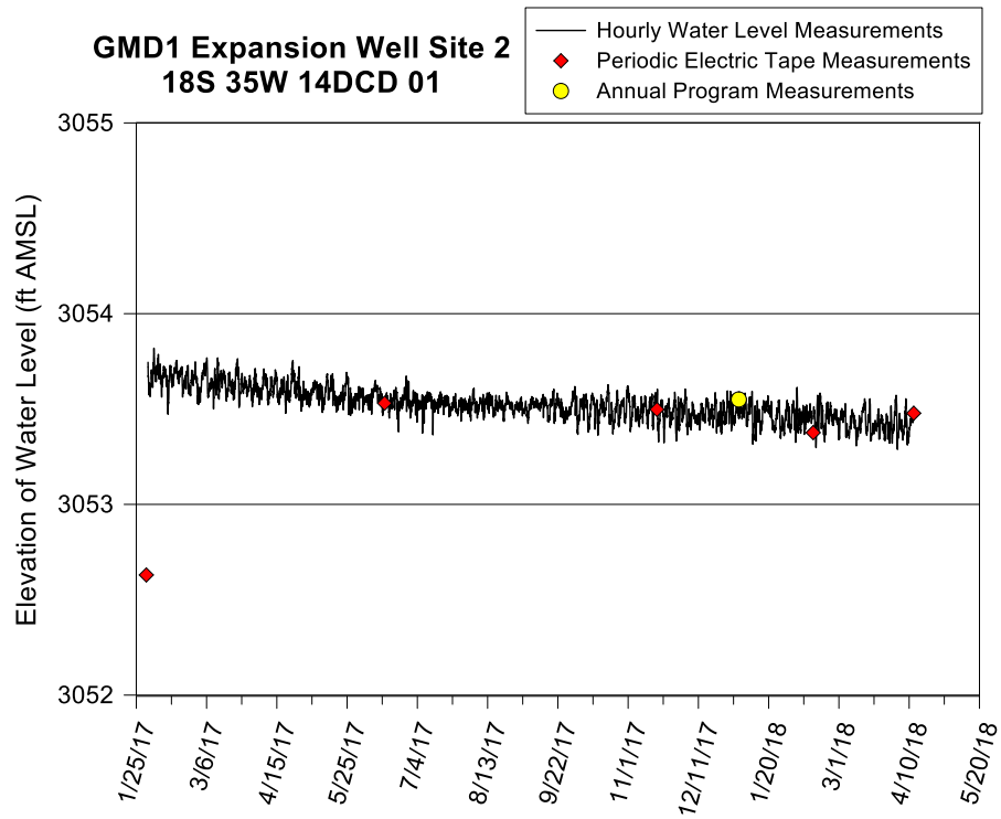
Figure 30—GMD1 Expansion Site 2 well hydrograph—total data run to 4/12/18. A water-level elevation of 3,053 ft corresponds to a depth to water of 118 ft below lsf. Bottom of well is 130.9 ft below lsf (elevation of 3,040.1 ft). First electric-tape measurement may be a transcription error.
