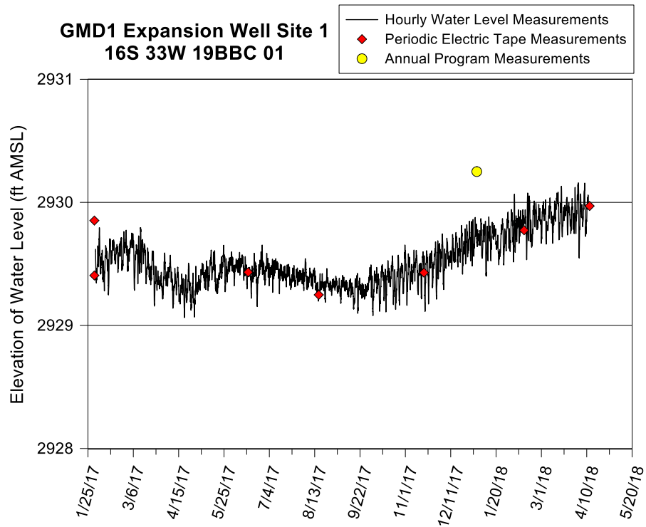
Figure 29—GMD1 Expansion Site 1 well hydrograph—total data run to 4/12/18. A water-level elevation of 2,930 ft corresponds to a depth to water of 168 ft below Isf. Bottom of well is 193.2 ft below Isf (elevation of 2,904.8 ft).
