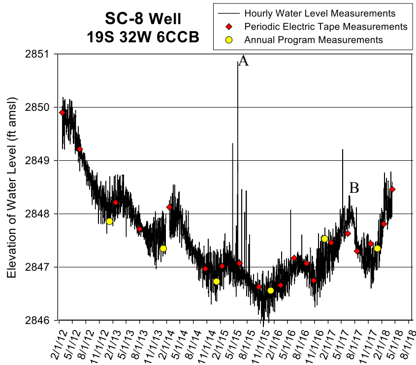
Figure 28—SC-8 well hydrograph—total data run to 4/12/18. A water-level elevation of 2,847 ft corresponds to a depth to water of 89 ft below Isf. Bottom of well is approximately 102 ft below Isf (elevation of 2,835 ft). Transducer measurements have been corrected from earlier reports for an incorrect offset parameter (Butler et al., 2017). A and B defined in text.
