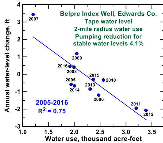
Figure 43—Correlation of annual water-level change in the Colby, SC-8, and Belpre wells with annual water use within a 1 or 2 mi radius around the wells during 2005–2016.
