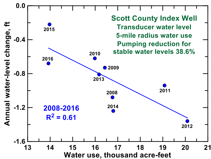
Figure 41—Correlation of annual water-level change based on transducer measurements in the Scott County index well with annual water use within a 5 mi radius around the well during 2008–2016 ( p=0.013 ).
