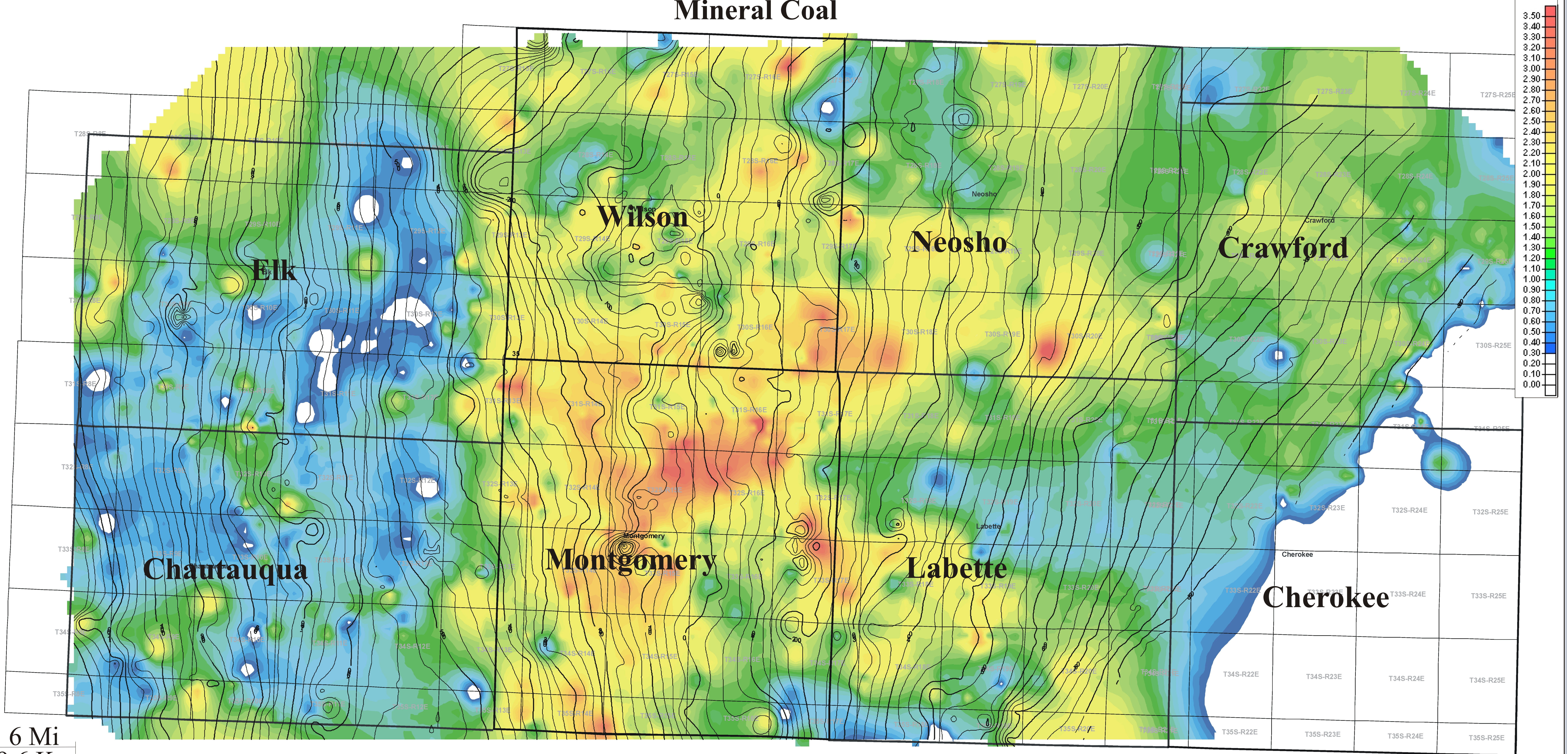
Isopach of Mineral coal (colors) overlain with contours on bottom Mineral coal structure (isopach CI: 0.10ft; structure CI: 25ft)
