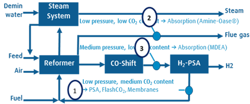
Figure 5.2. CO 2 capture in steam-methane reformer (SMR) based H 2 plants: Solvent, PSA/VSA & membrane applications
