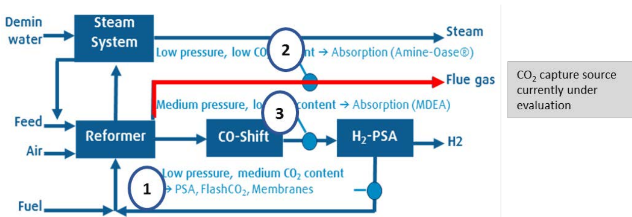
Figure 5.9. CO 2 Capture in Steam-methane reformer (SMR) based H 2 plants: Solvent, PSA/VSA & membrane applications.
