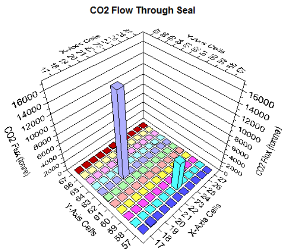
Figure 8: CO 2 flux through the Meramec limestone. The top figure shows total CO 2 leakage and its corresponding probability versus time. The bottom left figure shows one realization for the leakage rate assuming the entire seal is divided into 100 × 100 grid blocks. The bottom right figure shows the probability distribution for total CO 2 leakage.
