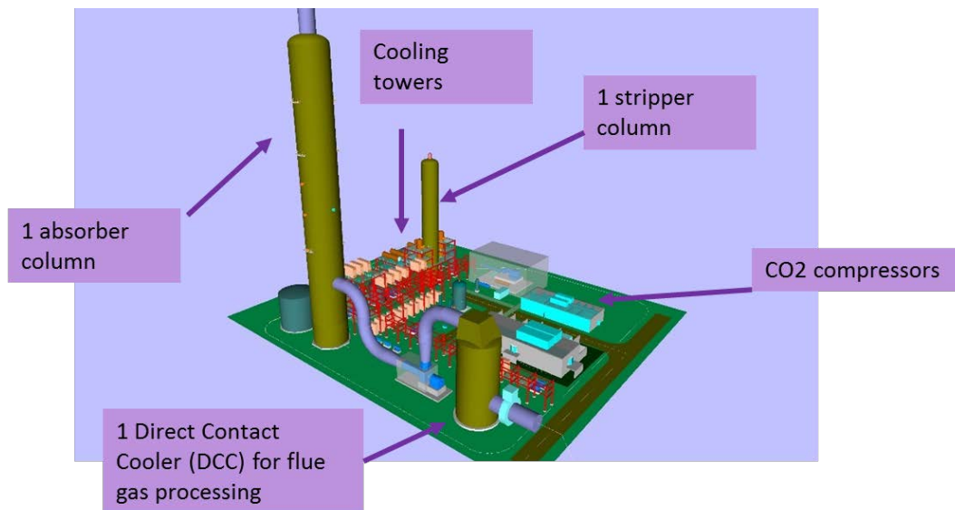
Figure 5.10. 3-D model of Linde-BASF post combustion capture plant designed for CHS refinery.
