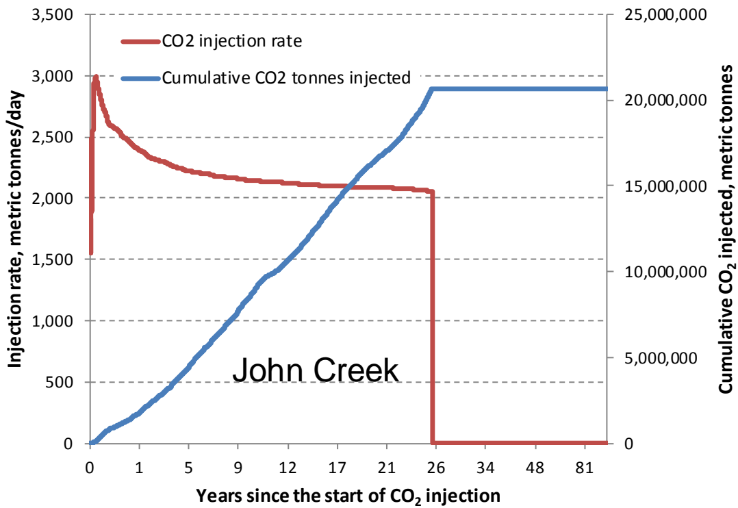
Figure 23. Cumulative CO 2 injected and CO 2 injection rate for Davis Ranch and John Creek sites. In both cases, the plots account for three wells completed at two intervals: Simpson and Arbuckle.
