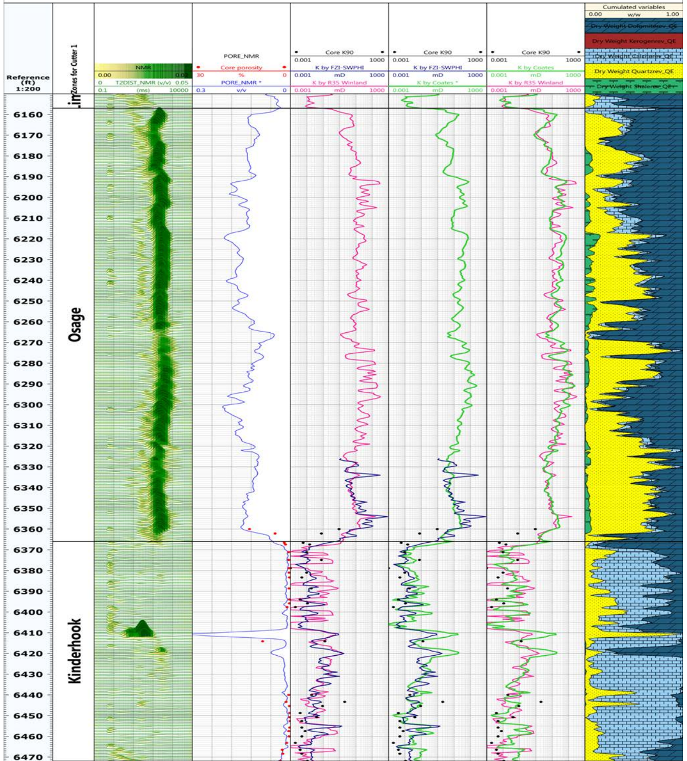
FIGURE 1: Calculated permeability by three methods compared to core in the Cutter-KGS *1 well. Figure 1 extends to the following three pages.
