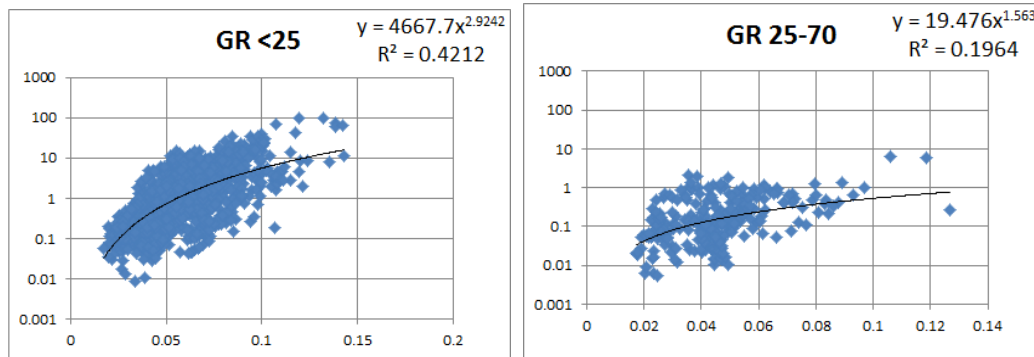
Figure 16: K-PHI relationship for GR<25 and for GR 25-70.
