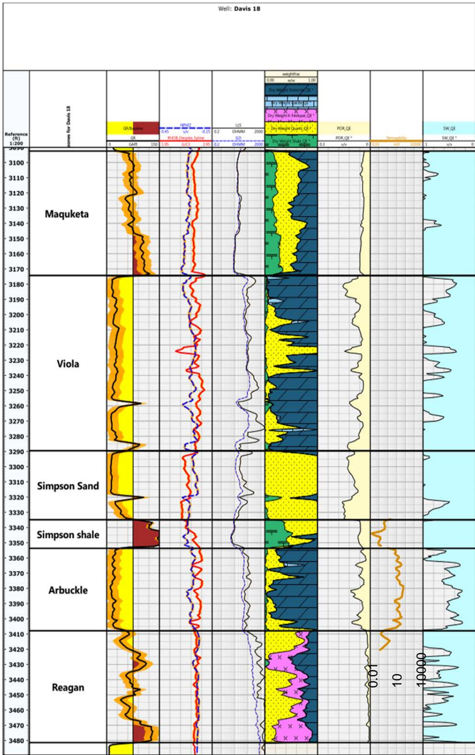
Figure 17. Log analysis and permeability by Neural Network in Davis 18. Permeability is in the second track from the right. Log scale ranges from 0.01 to 10,000 mD.
