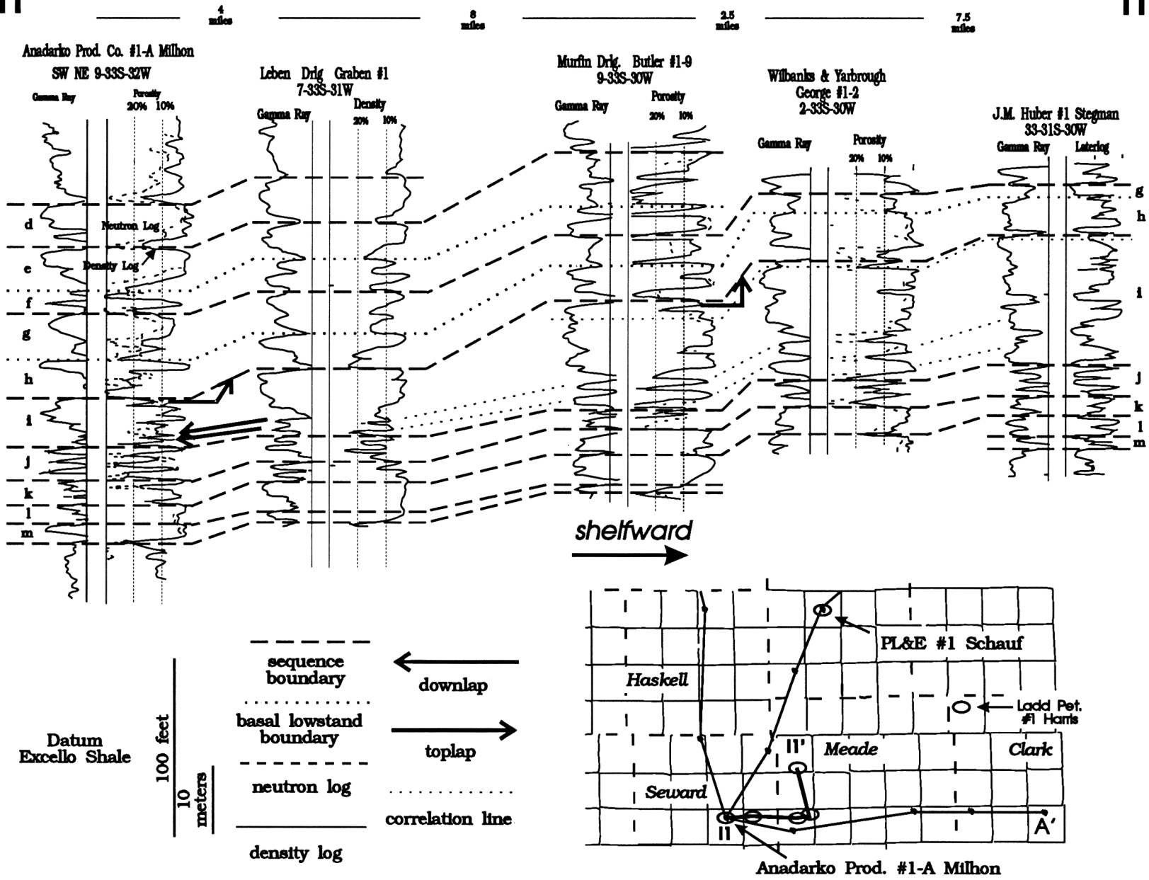
FIGURE 31—CROSS SECTION I1—I1' DISPLAYING INTRASEQUENCE CORRELATIONS and the thickening of sequence i from the lower shelf to the mid-shelf.
